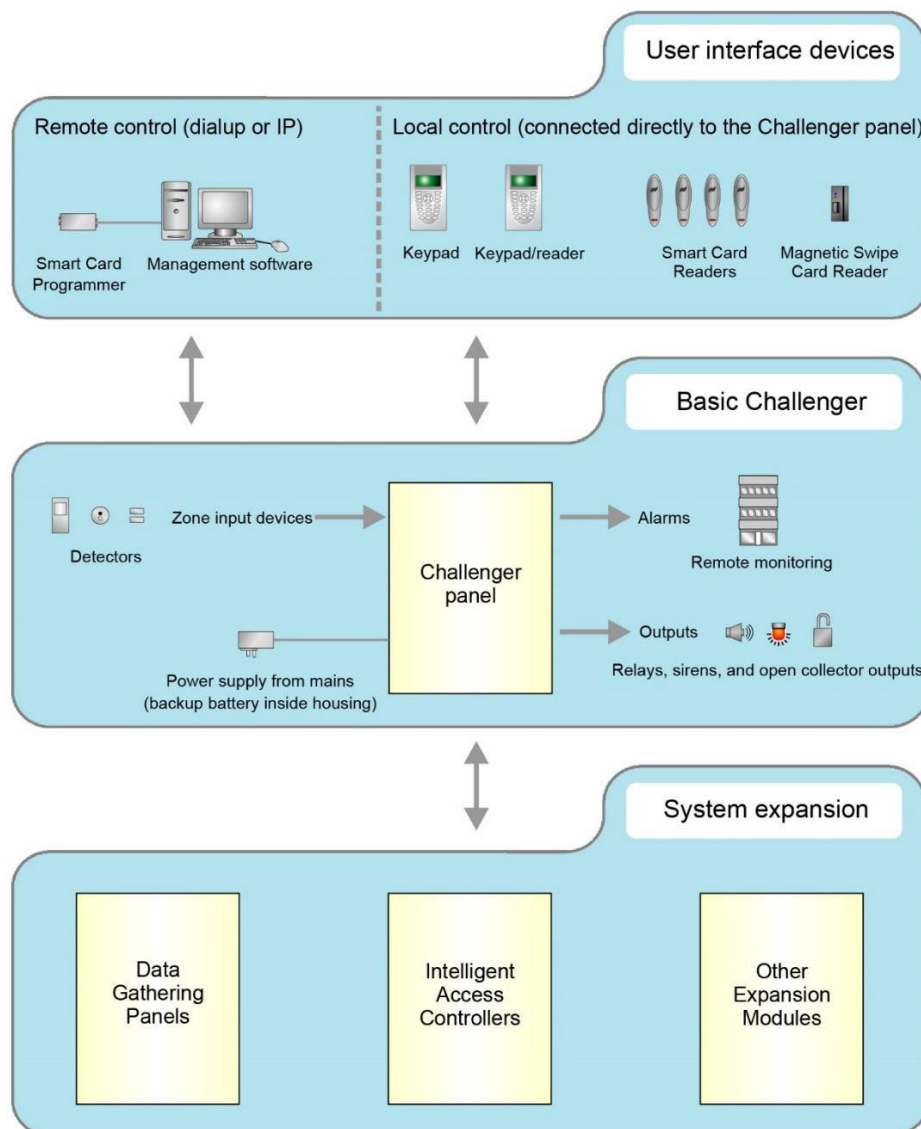
Figure 1: Challenger system overview
