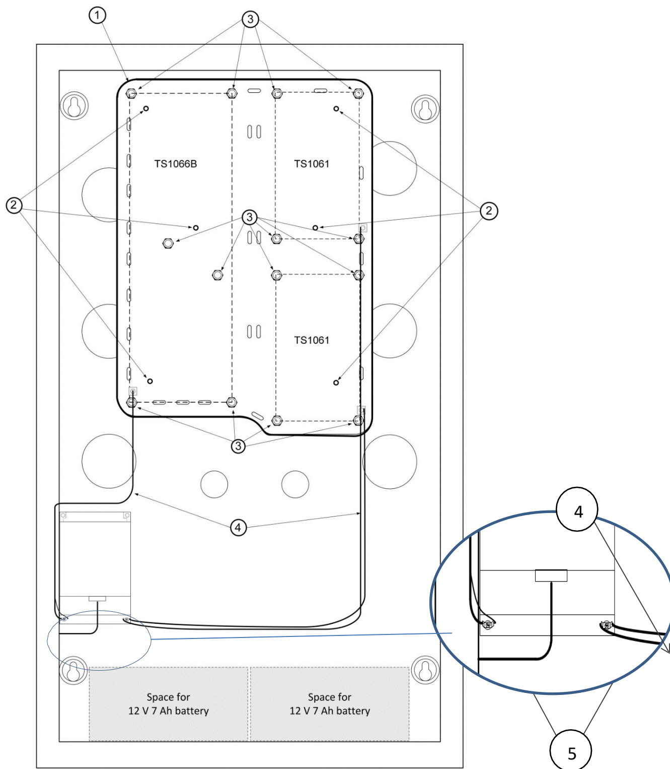
Figure 2: TS1066P installation in enclosure
