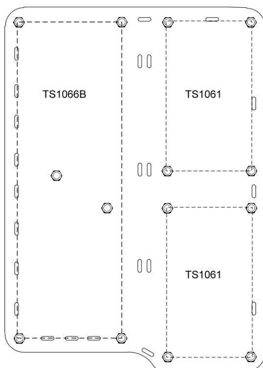
Figure 1: TS1066P board mounting locations
