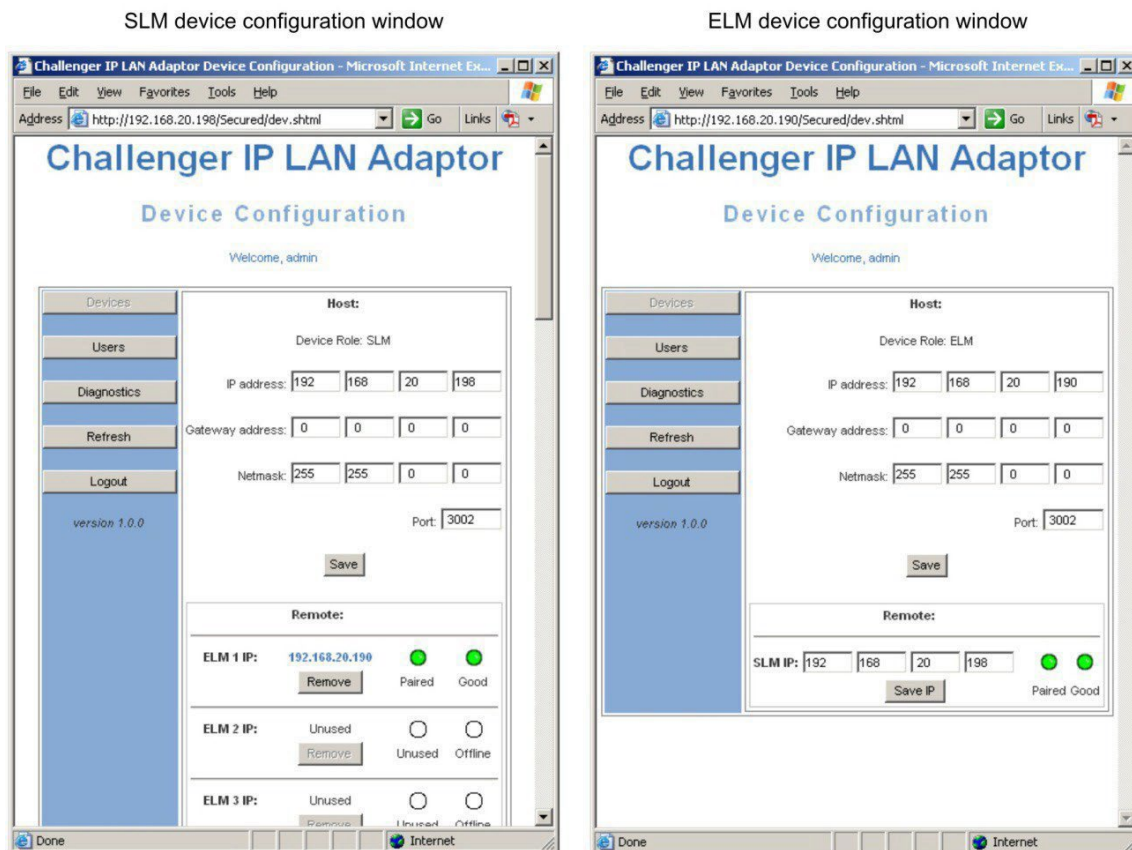
Figure 8: Device Configuration windows for SLM and ELM
