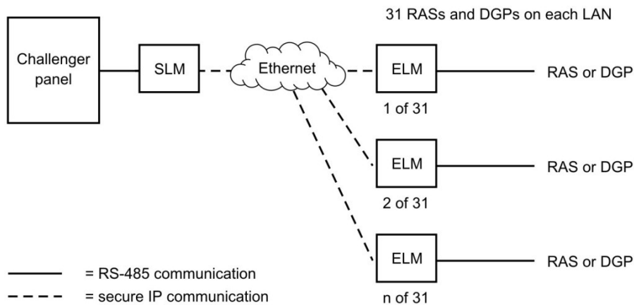
Figure 3: One SLM used with multiple ELMs
