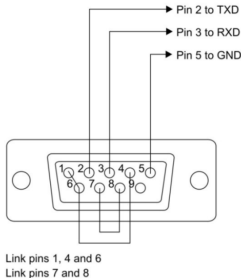
Figure 6: Wiring details for DB9 connector
