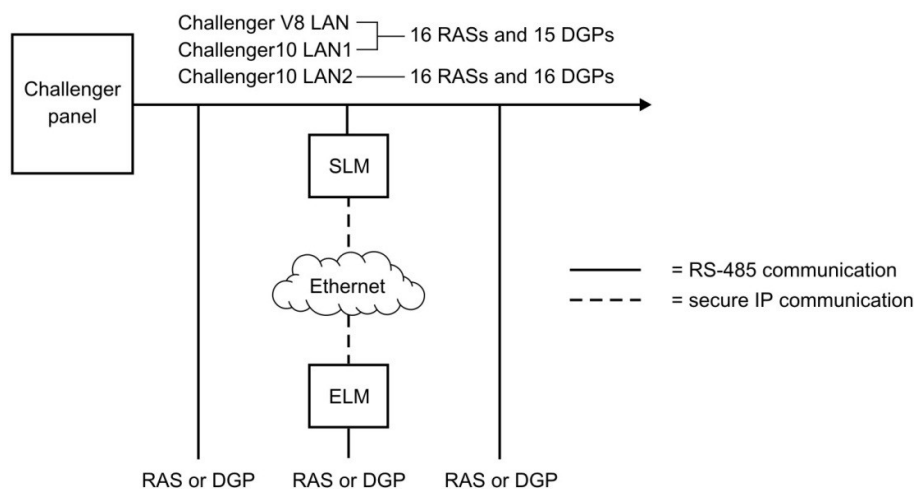
Figure 1: One SLM and one ELM connecting a single LAN device
