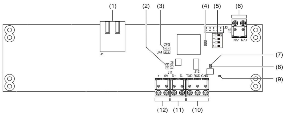
Figure 4: TS0098 Challenger IP LAN Adaptor general layout
